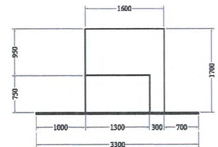
VIEW D
